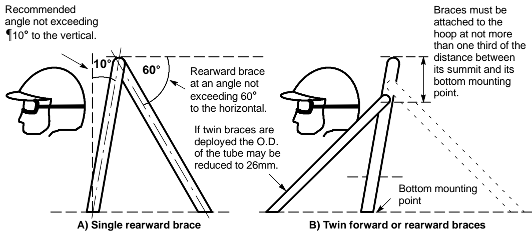
Fig 2. Roll over protection structure bracing guidelines
